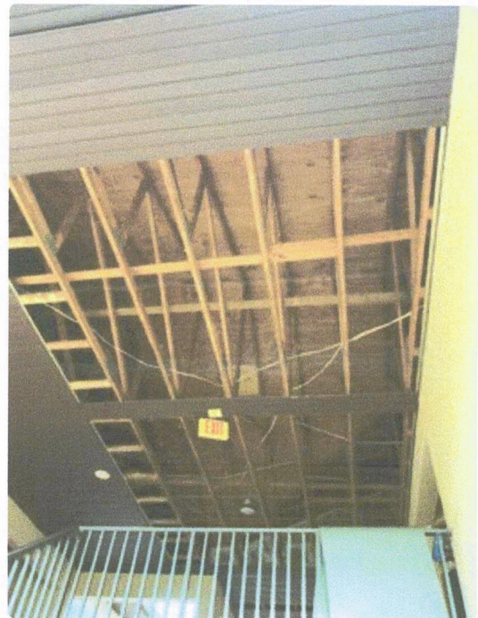
Trusses are 24" on center.
